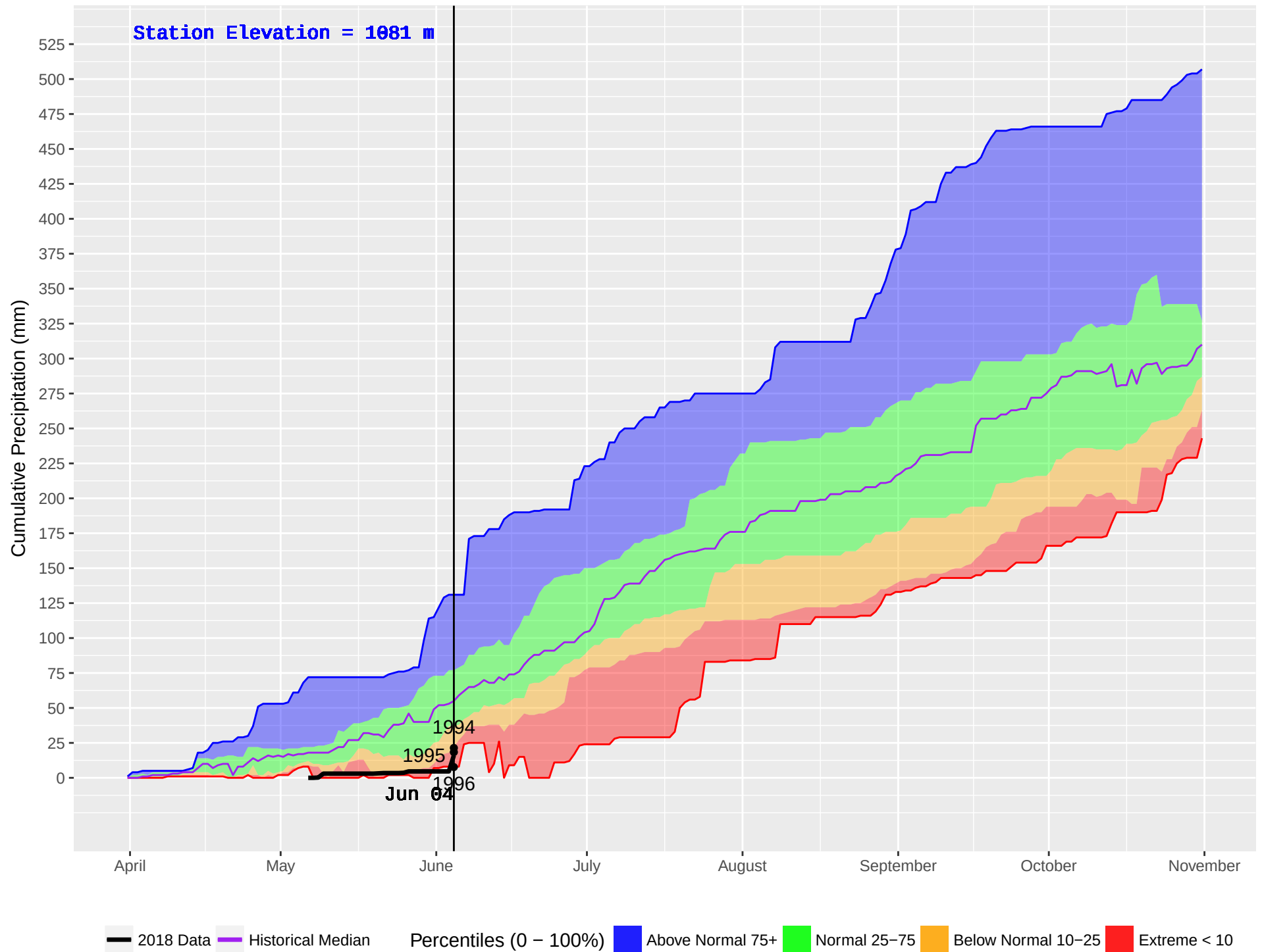
GAVIN (227) : Historical (1981–2016) and Current (2018) Noon Cumulative Precipitation
