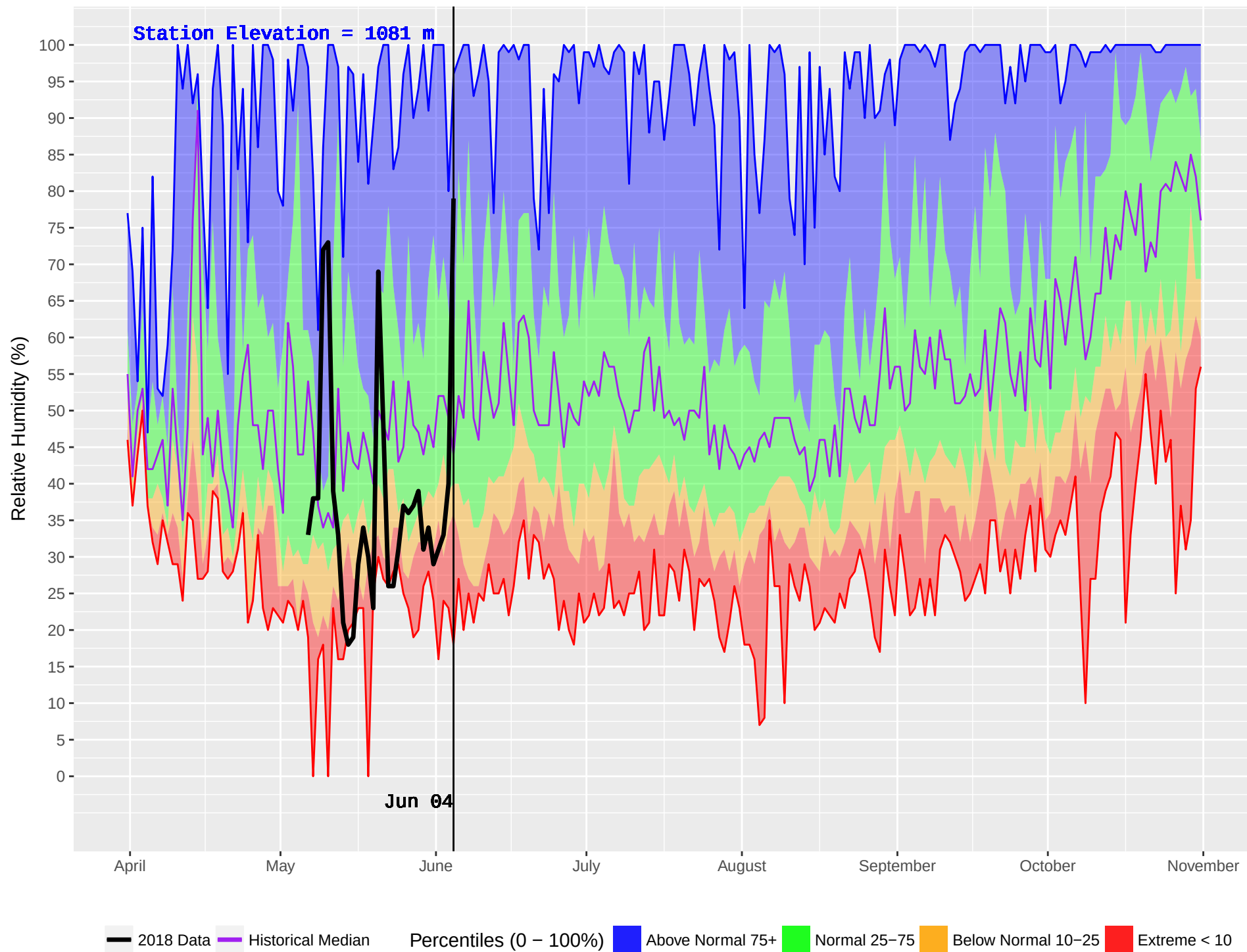
GAVIN (227) : Historical (1981–2016) and Current (2018) Noon Relative Humidity
